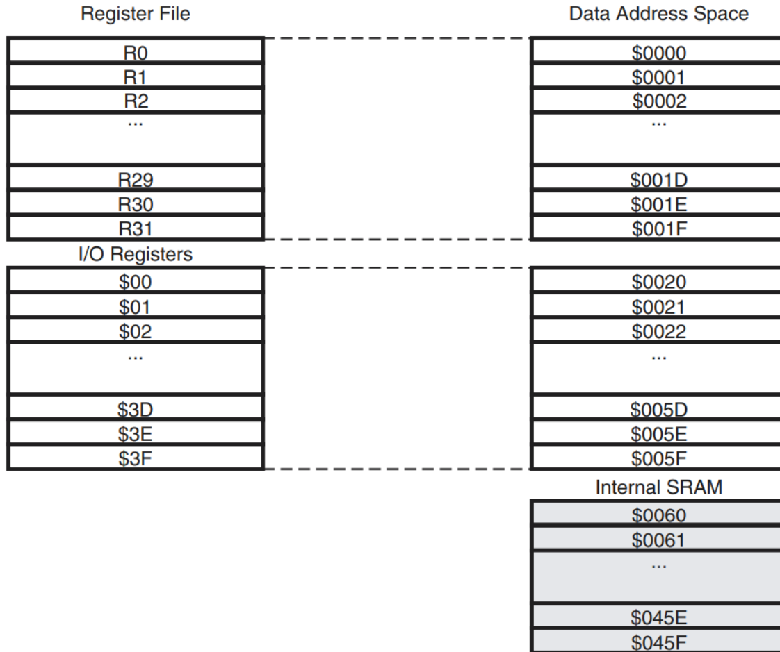
Data Memory Map
