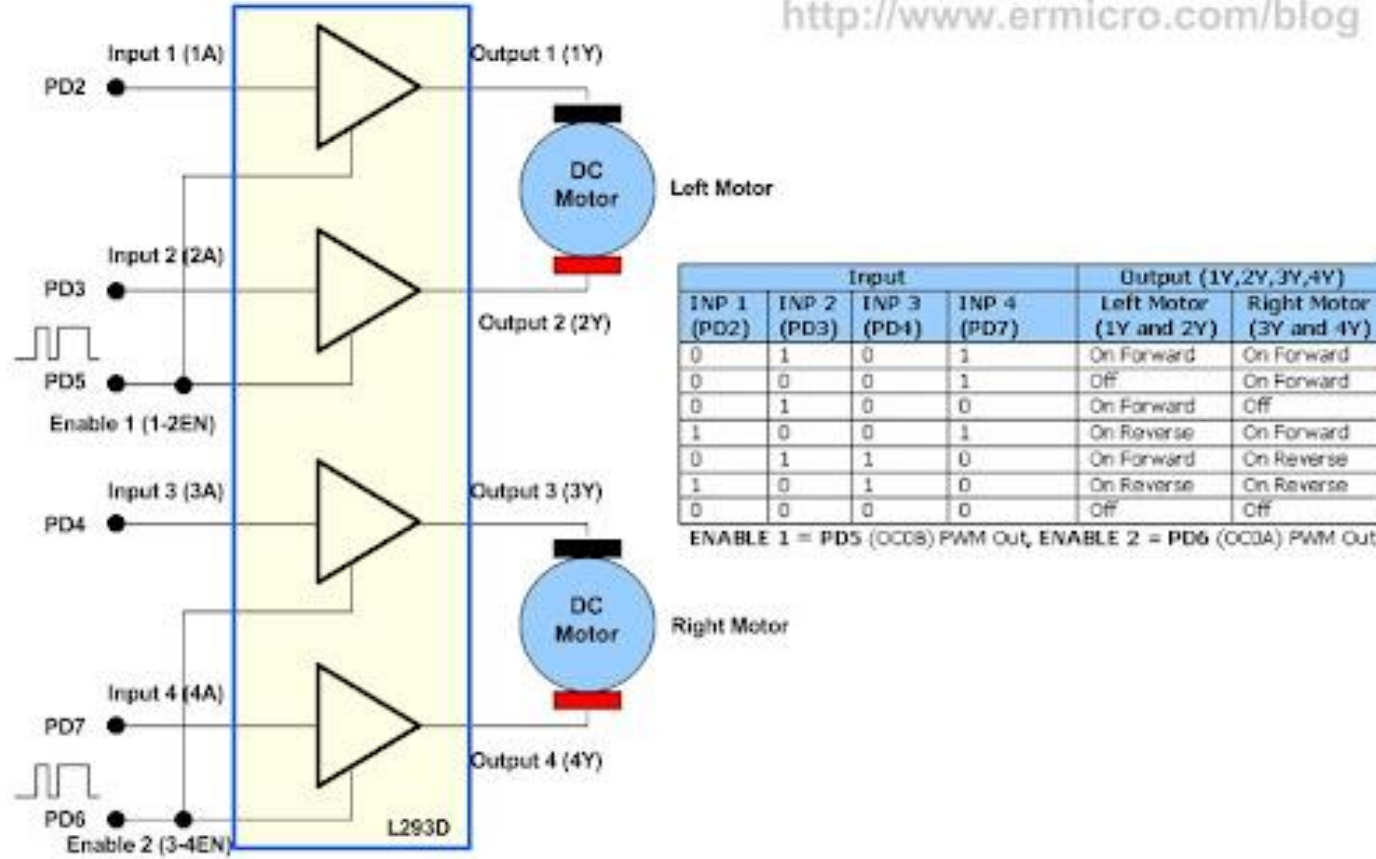
BRAM II L293D Driver Logic Control
